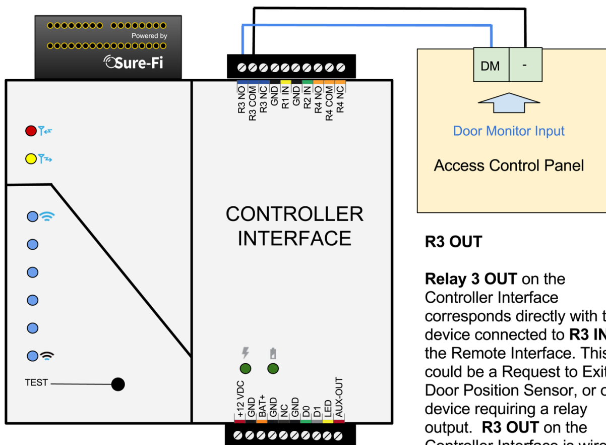
Figure 10: Relay 3 Wiring Controller Interface
