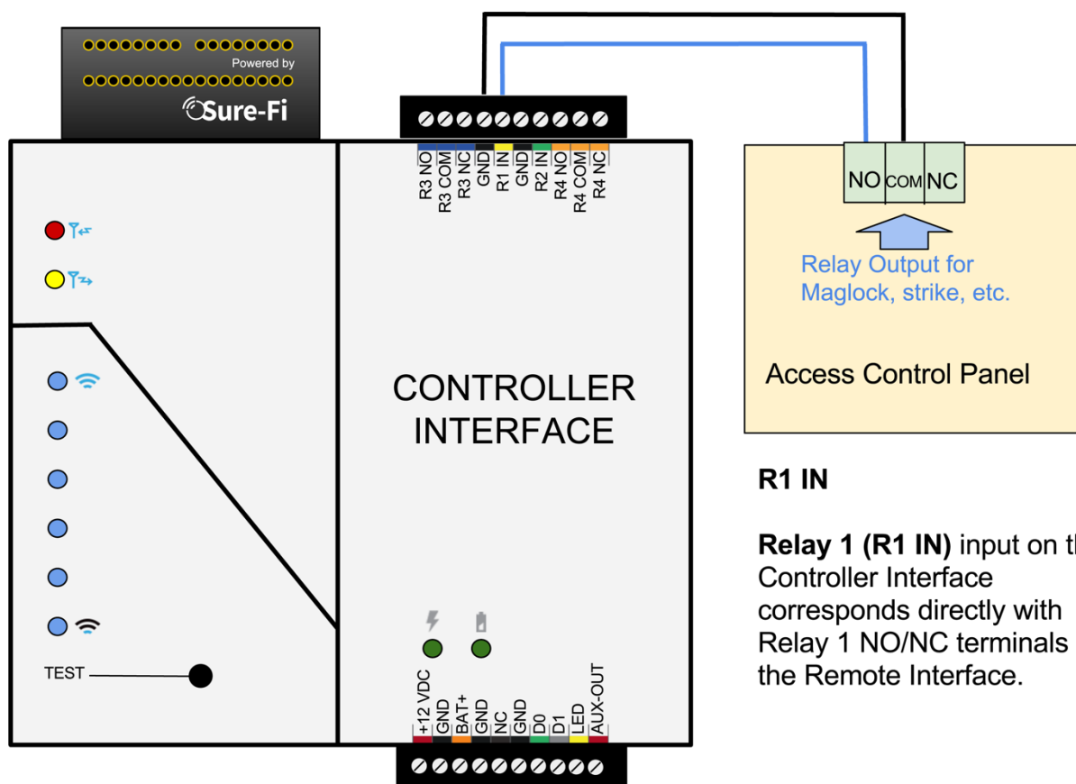
Figure 8: R1 IN Wiring Controller Interface
