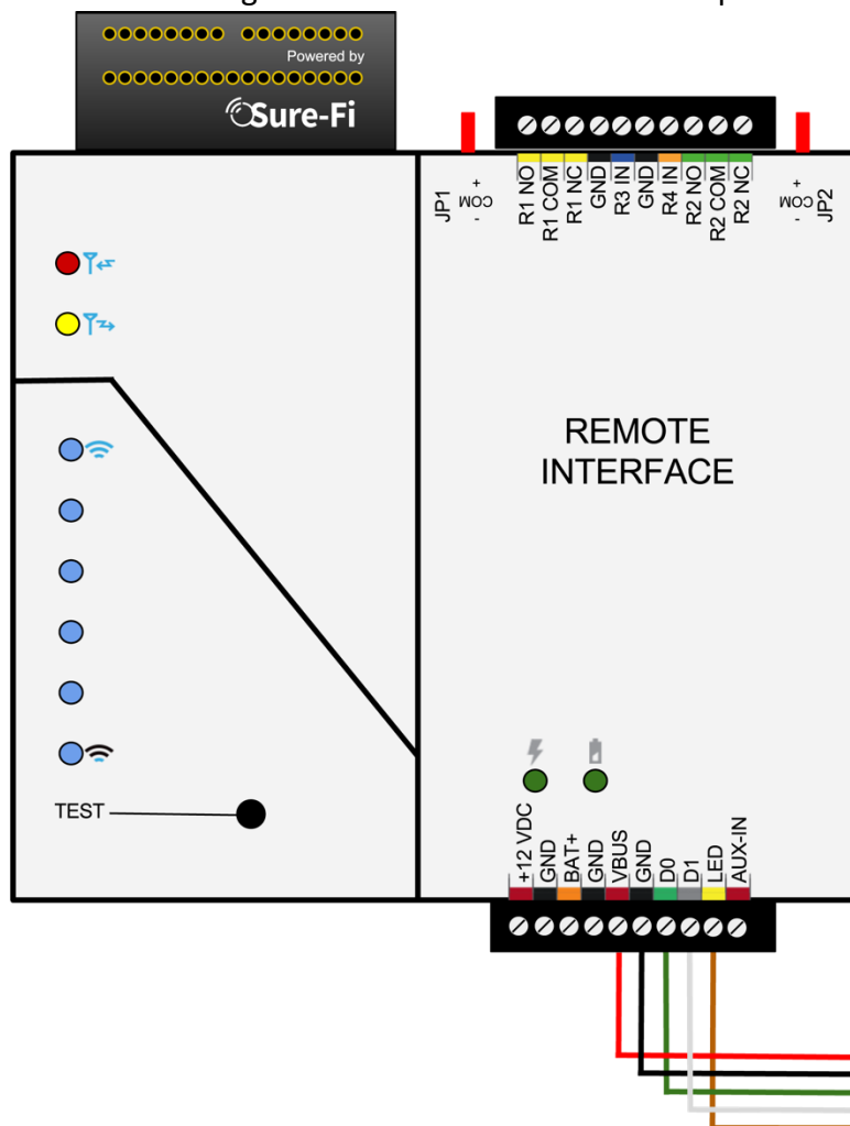
Figure 5: Wiegand Wiring Remote Interface
