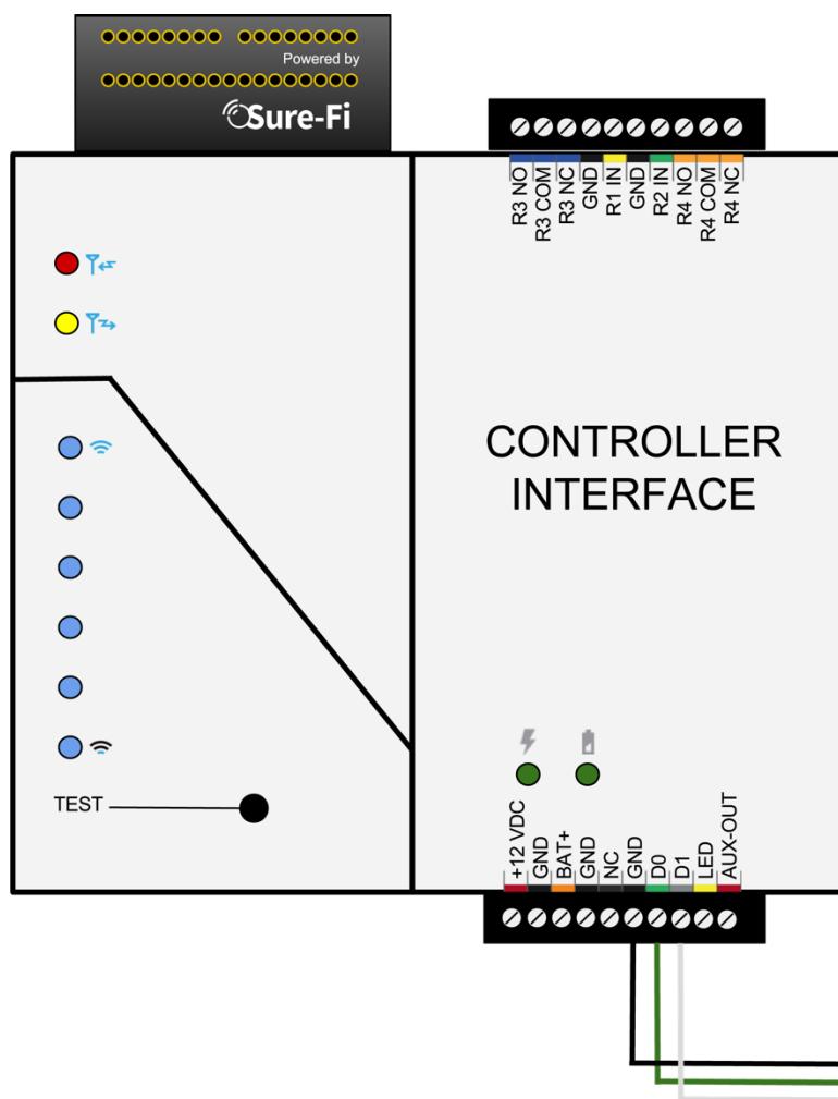
Figure 6: Wiegand Wiring Controller Interface
