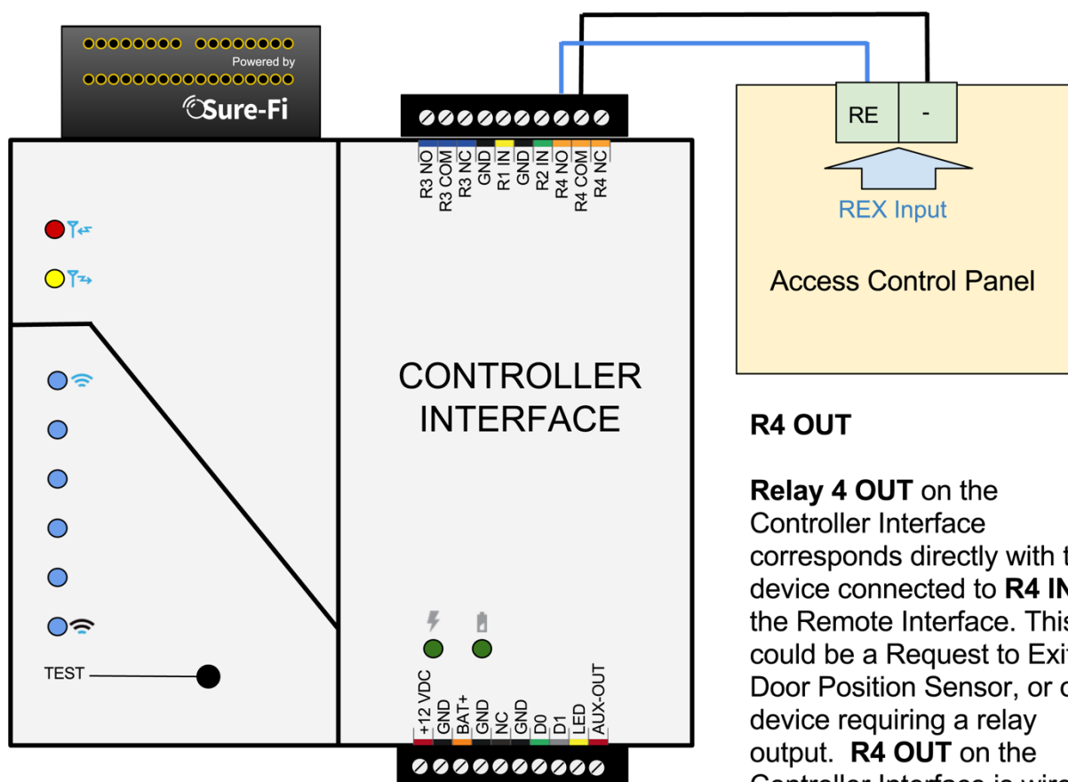
Figure 12: Relay 4 Wiring Controller Interface
