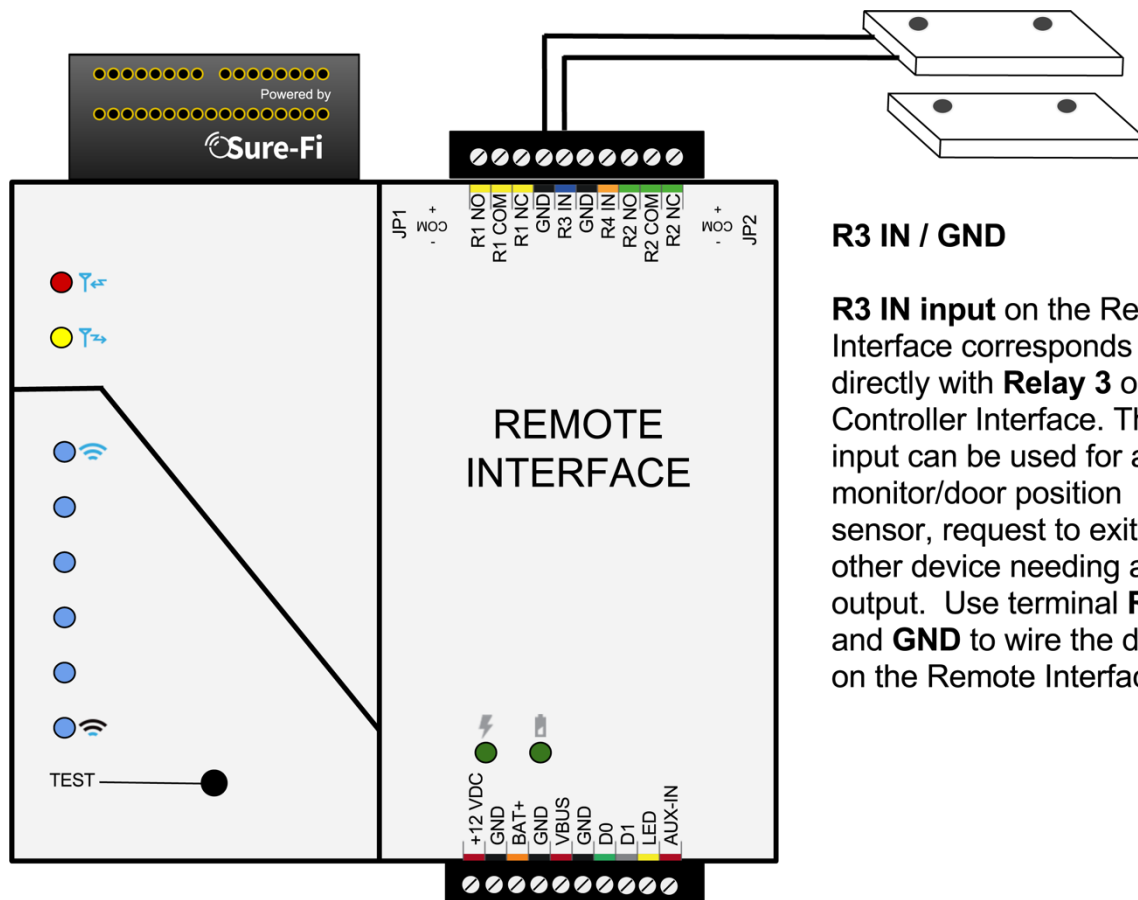
Figure 9: R3 IN Wiring Remote Interface
